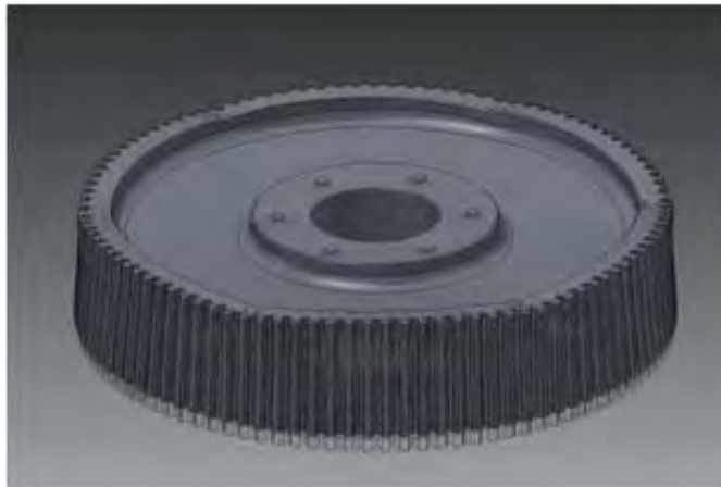
Figure 15. Deformations seen from a different view of a simulation of a gear by horizontal charging
