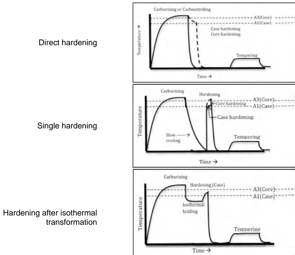
Figure 18. Positive effect due to choice of hardening procedure. The differences in hardening procedures can have a great effect on the outcome of a gear
