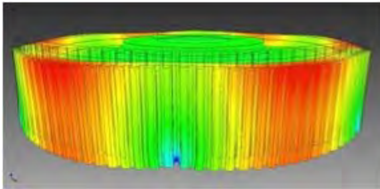
Figure 26. Simulation of the hardening distortion of a spur wheel gear with horizontal charging, stress marks shown with different colors
